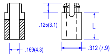
FIG. 3 SERIES 07-14 .234±.003 (5.9±0.08) HOLE DIA. .062 (1.6) MATERIAL THICKNESS.
