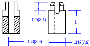
FIG. 2 SERIES 07-13 .234±.003 (5.9±0.08) HOLE DIA. .062 (1.6) MATERIAL THICKNESS.
