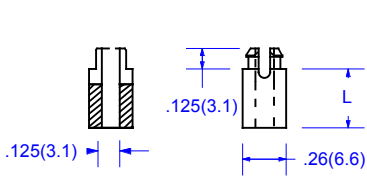
FIG. 1 SERIES 07-12 .187±.003 (4.7±0.08) HOLE DIA. .062 (1.6) MATERIAL THICKNESS.
