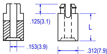
FIG. 5 SERIES 07-16 .234±.003 (5.9±0.08) HOLE DIA. .062 (1.6) MATERIAL THICKNESS.
