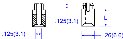
FIG. 4 SERIES 07-15 .187±.003 (4.7±0.08) HOLE DIA. .062 (1.6) MATERIAL THICKNESS.
